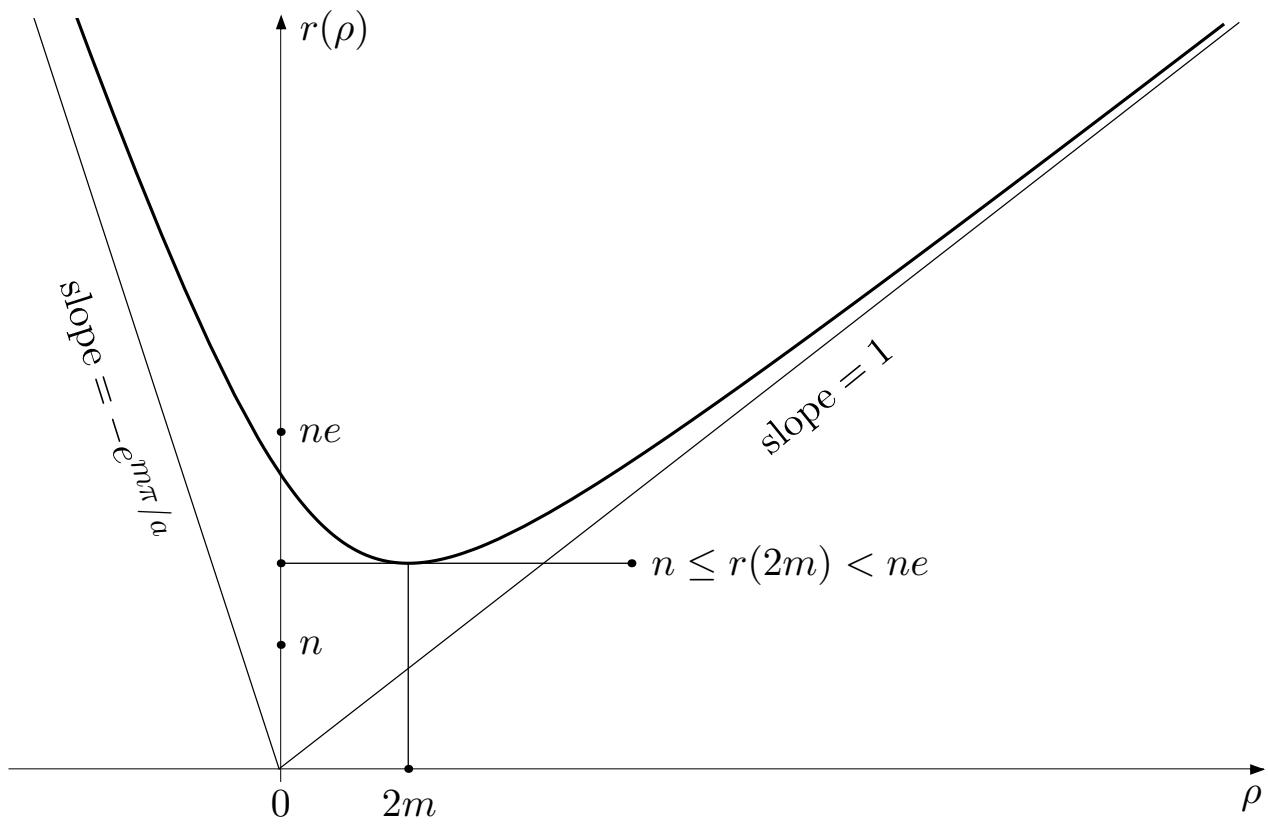
Graph of the radius function r for generic values of m and n .
