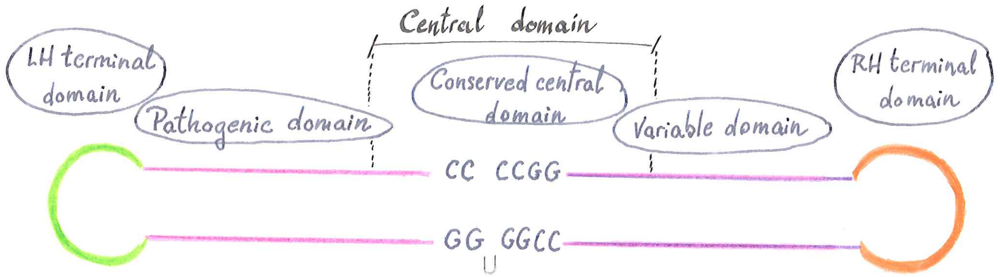
Scheme of a Pospiviroid
