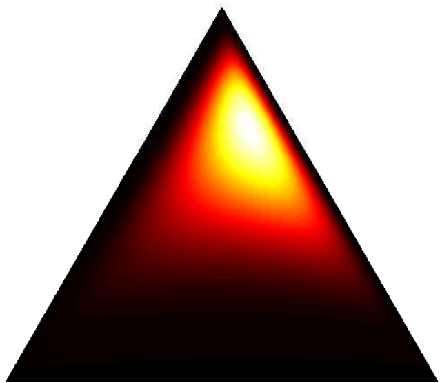
Logistic Normal
