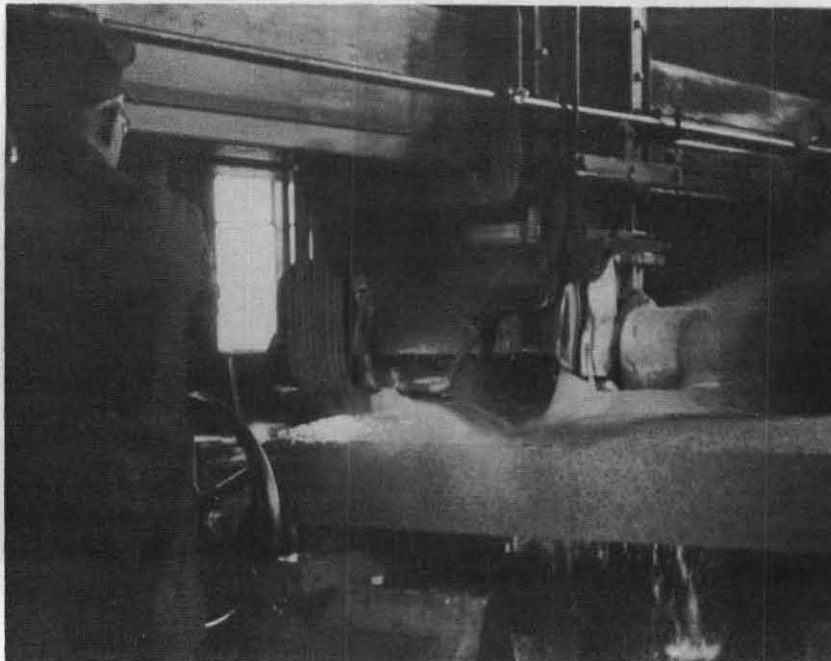
FIGURE 19. Contour machine making a curved smooth surface on a granite slab. Water used to cool the wheel also keeps down the dust. (1955.)
