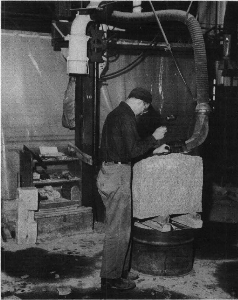
FIGURE 26. Hand-pitching, one of the oldest hand operations, is still being employed in modern stone-sheds. (1957.)
