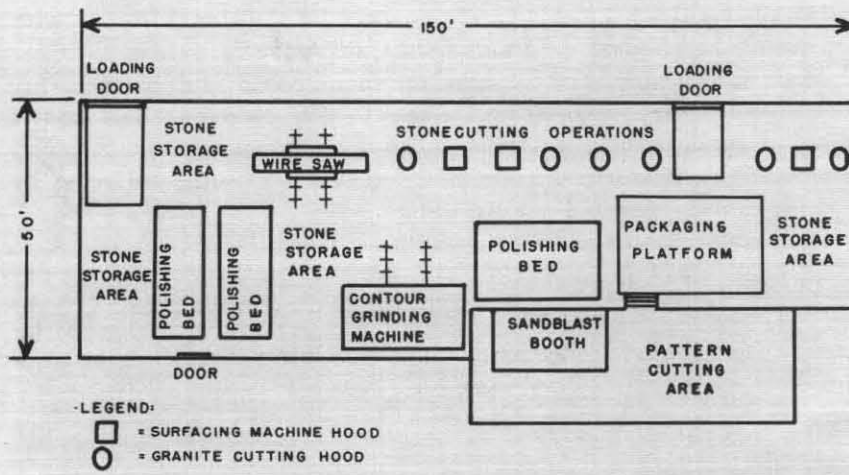
FIGURE 16. Floor plan of typical granite cutting shed employing about 25 persons. (1955.)
