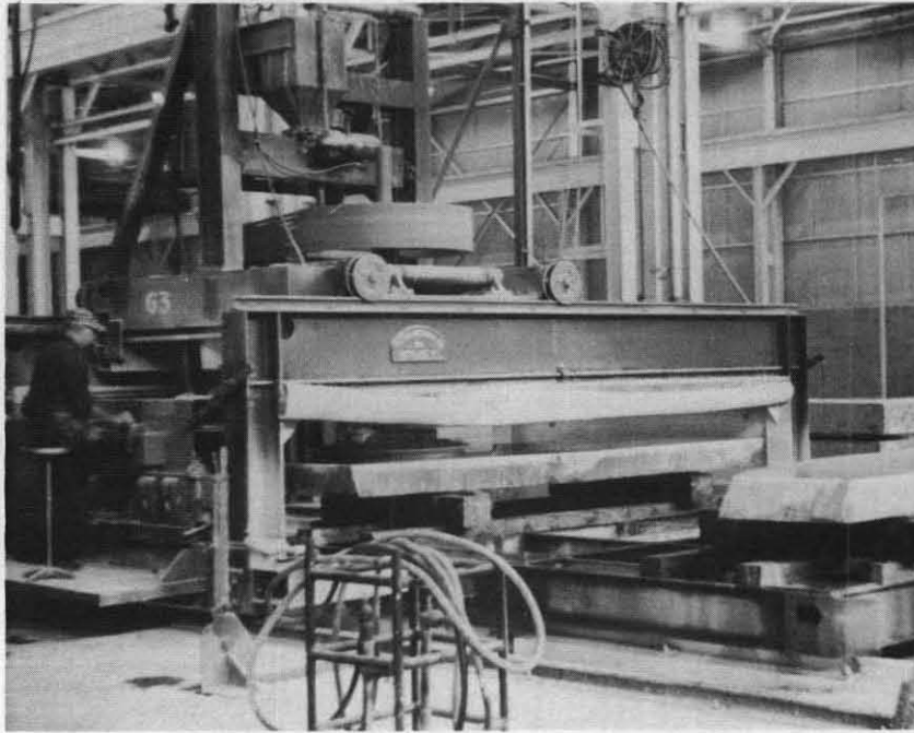
FIGURE 18. Traveling bed polishing machine in operation in a new shed since 1956.
