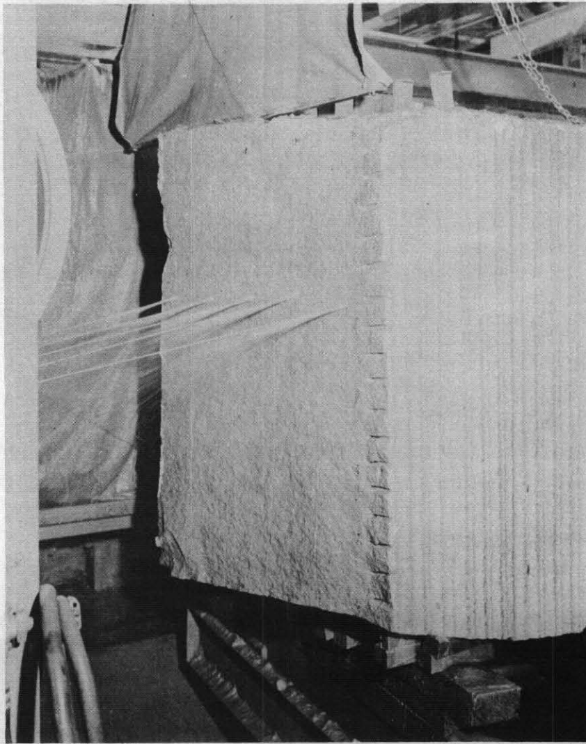
FIGURE 24. Multiple wire saw. Note abrasive slurry leaving wire. (Courtesy of Smith, Whitcomb & Cook Co., 1955.)
