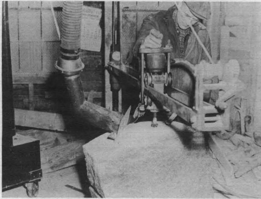
FIGURE 6. This picture, taken in 1936, shows that dust from a baby surfer can be effectively controlled by local exhaust ventilation. However, the hood is only effective when used close to the bit.
