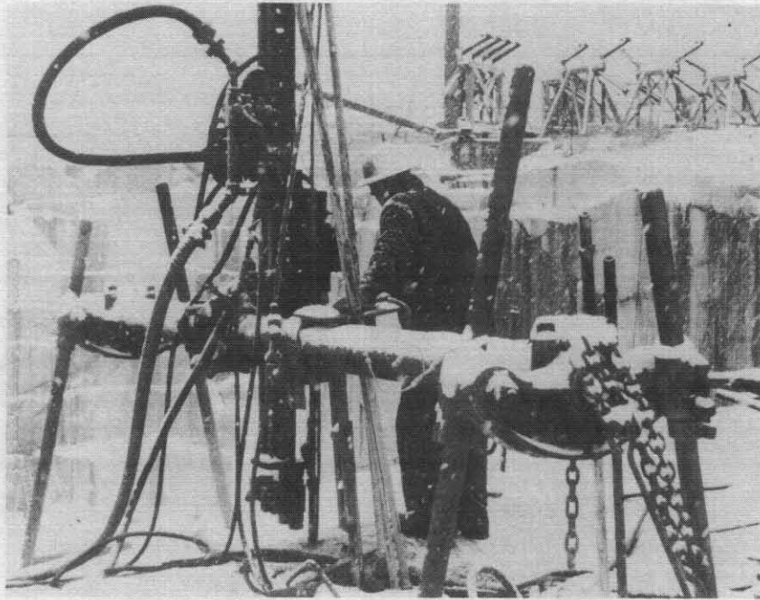
FIGURE 10. Wet drilling with leyner in winter. Heated water is being used. (1955.)
