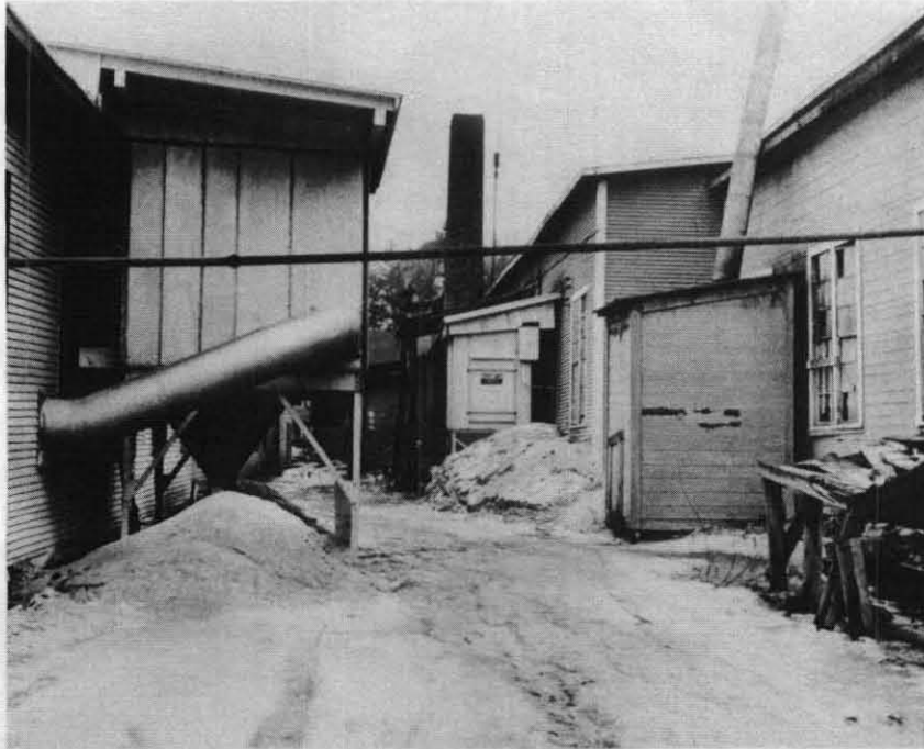
FIGURE 5. Early attempts to collect the dust generated from granite cutting operations in sheds. To the right is a settling chamber with high stack to prevent dust from re-entering the shed. To the left is a more modern cloth bag dust collector. Prior to 1948, air discharged from the collector was recirculated in most sheds. (About 1937.)
