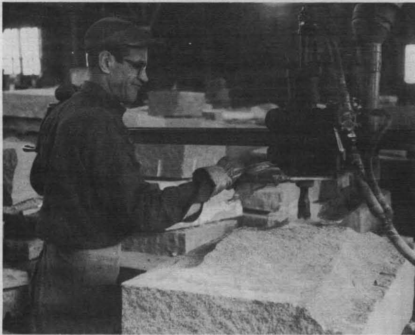
FIGURE 23. Baby surfer in operation. Note exhaust hood is permanently attached to the head and remains close to the bit. See figure 6 for contrast with earlier model. (1955.)
