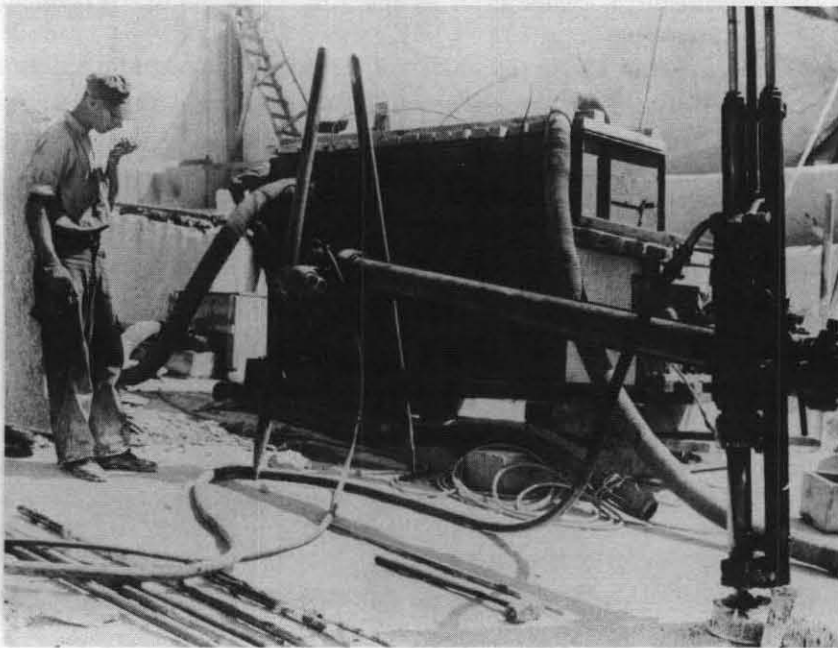
FIGURE 13. One of the several types of local exhaust systems for controlling dust in the quarries about 1937. Note collar around drill at lower right and flexible hose. None of these early exhaust systems proved successful and as a consequence drilling was usually done without benefit of dust control until about 1950.
