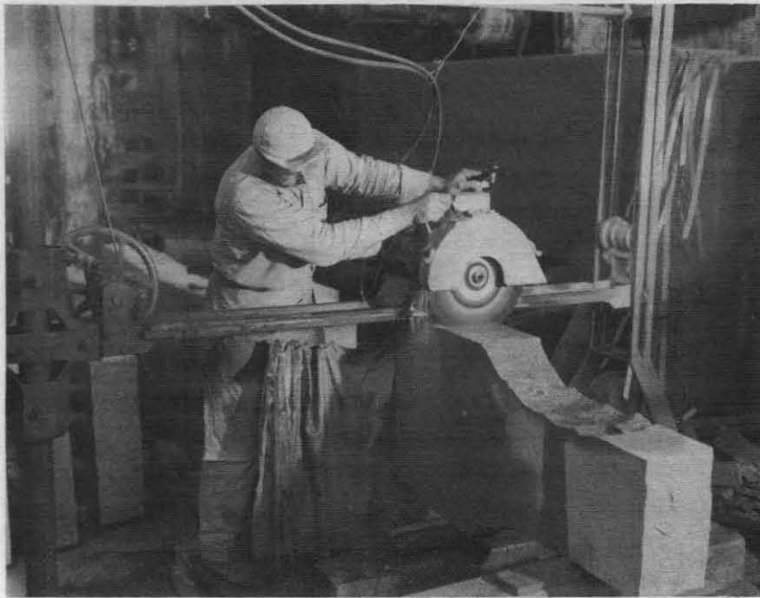
FIGURE 20. Diamond cutting saw. Note water spray. (Courtesy of Smith, Whitcomb & Cook Co., 1955.)
