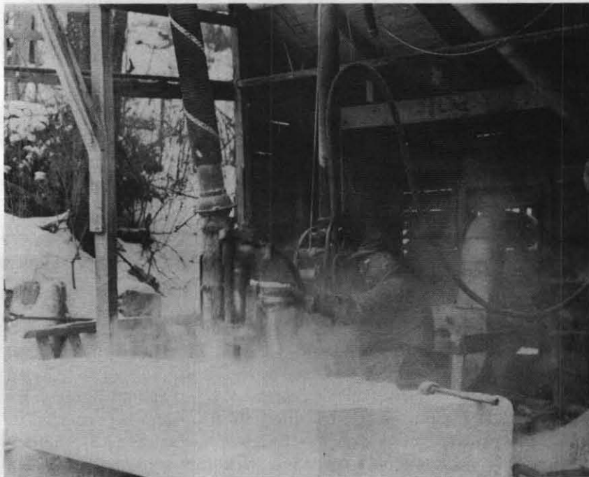
FIGURE 4. Early type of local exhaust for surfacing machine in an open shed. From the amount of visible dust the local exhaust was either not in operation or not effective. A large blower, in background, was not connected to exhaust ducts and was apparently used to remove dust from the general work area. (About 1936.)
