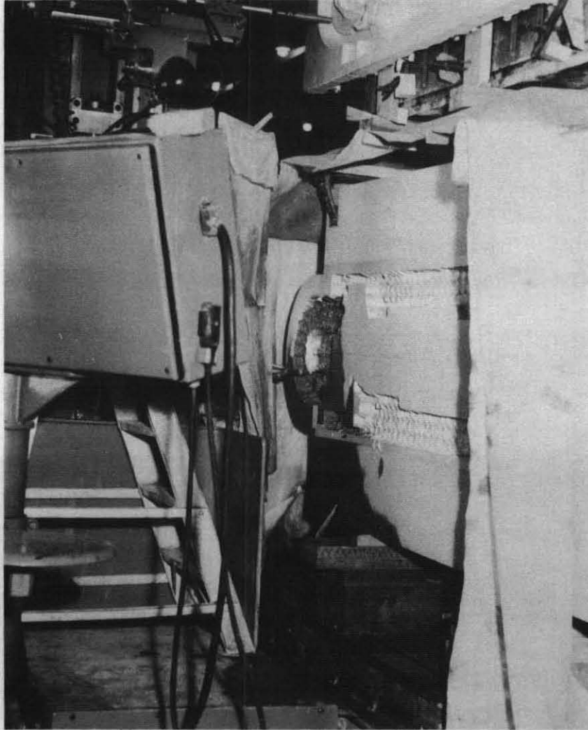
FIGURE 21. Profiling machine in operation in a new shed since 1956. Stylus following contours in plastic model at top controls the rotating diamond tool in cutting out the design.
