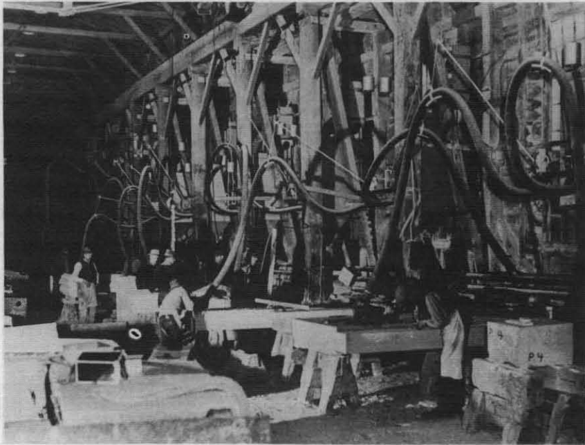
FIGURE 7. Interior view of a granite shed showing individual dust collectors attached to flexible hoses and exhaust hoods. (About 1937.) These units were gradually replaced by one or more larger central dust collectors.
