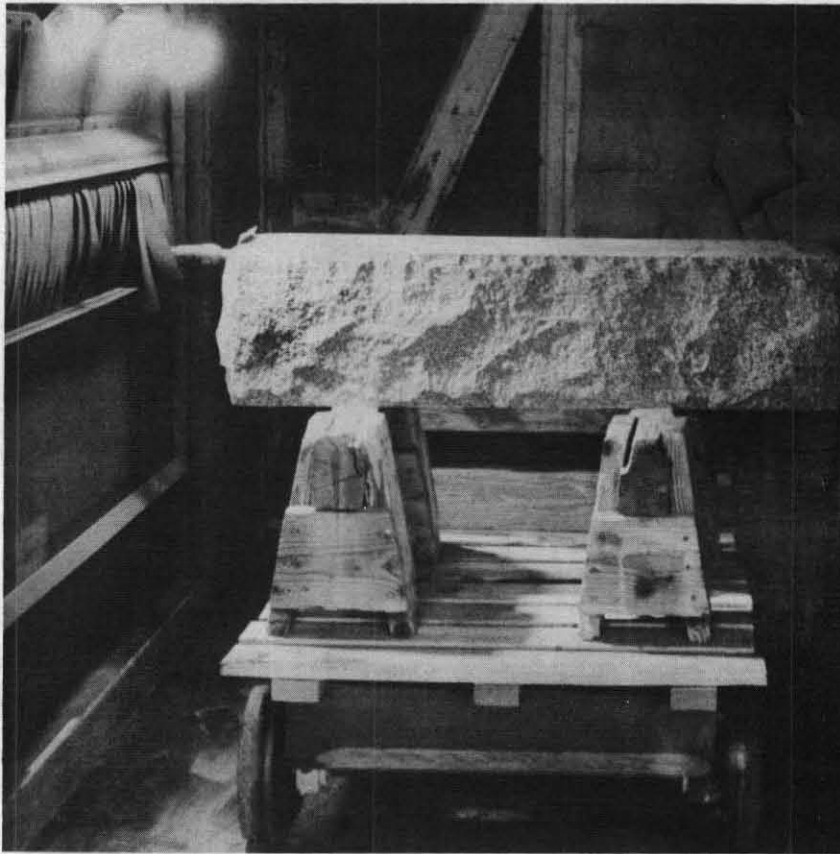
FIGURE 29. Inside an exhausted sandblast booth. Operator working from behind window is sandblasting an inscription on end of slab. (1955.)
