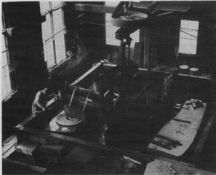
FIGURE 17. Type of polishing machine in use for over 30 years. (1955.)
