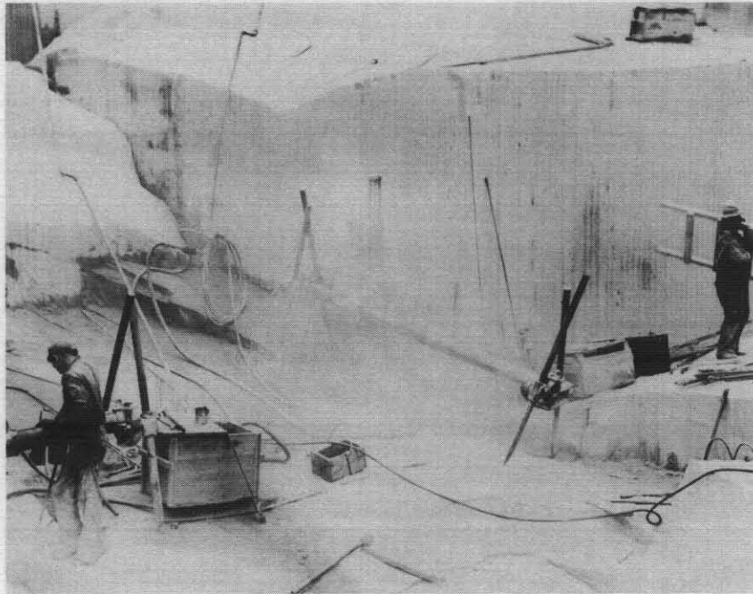
FIGURE 11. Leyner bar drilling without dust control. Operator in background is barely visible through dust cloud. (About 1936.)
