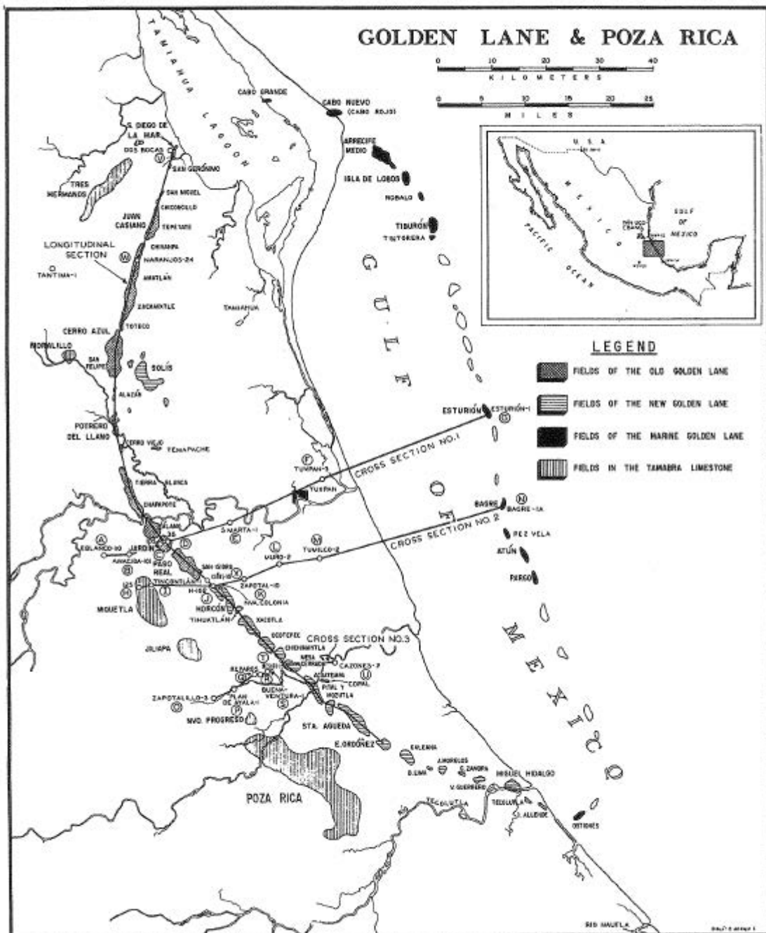
FIG. 1.—Index map, Golden Lane fields, eastern Mexico, showing lines of cross sections in Figures 6-8. Individual wells used in cross sections (A-V) are listed in Table 1.
